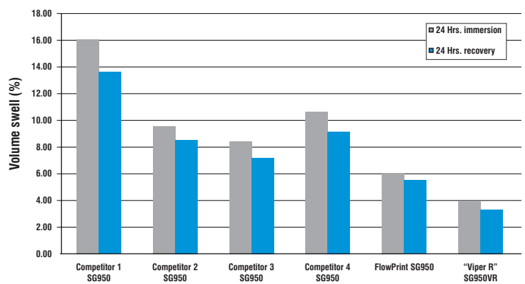
75 Shore A “Single green” Construction Volume Swell in Cyclohexanone
