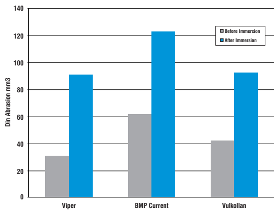
“Viper” Abrasion Resistance Comparison
