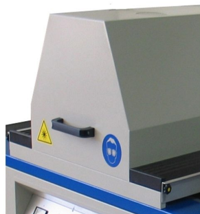
UV Lamp housing 100% closed equipped with crystal quartz glass so no heat is transmit to drying object
